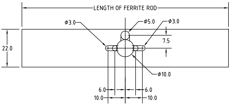
ANTENNA TUBE UNDERSIDE VIEW
