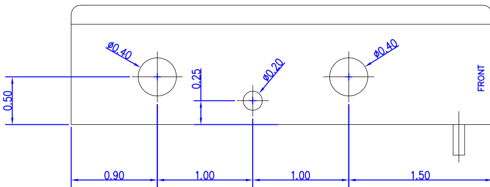
SIDE HOLES (VIEW FROM OUTSIDE THE BOX)
